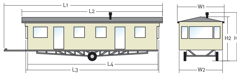
PRIMA-3 External dimensions for each model in the range
